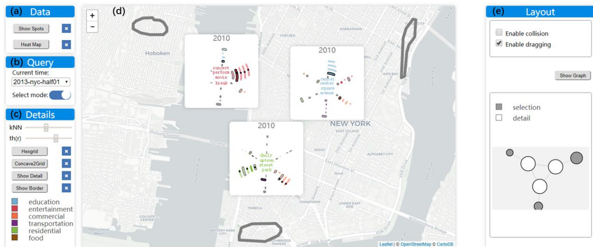
Figure 1: The interface of our system consists of (a) Data menu. Scatter plot and heatmap are provided for displaying the the distribution of data. (b) Query menu. Users can retrieve data at specific time, or enable the free selection mode to query an AOI (Area Of Interest). (c) The Details menu allows users to change parameters, view details of AOIs and refer the color legend. (d) Map view of the current time step. (e) In the Layout menu, users can adjust positions of details.
