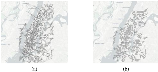
Figure 4: Cluster spots based on kNN graph. (a) Graph constructed by connecting spots with its 10NN neighbors. (b) Communities are delimited by concave boundaries.
